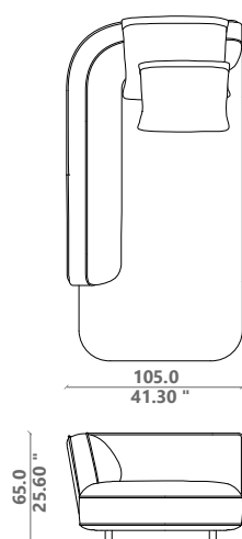
ALCL1DX Sofa chaise longue 01 dx
