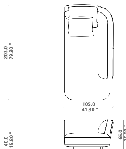
ALCL1SX Sofa chaise longue 01 sx
